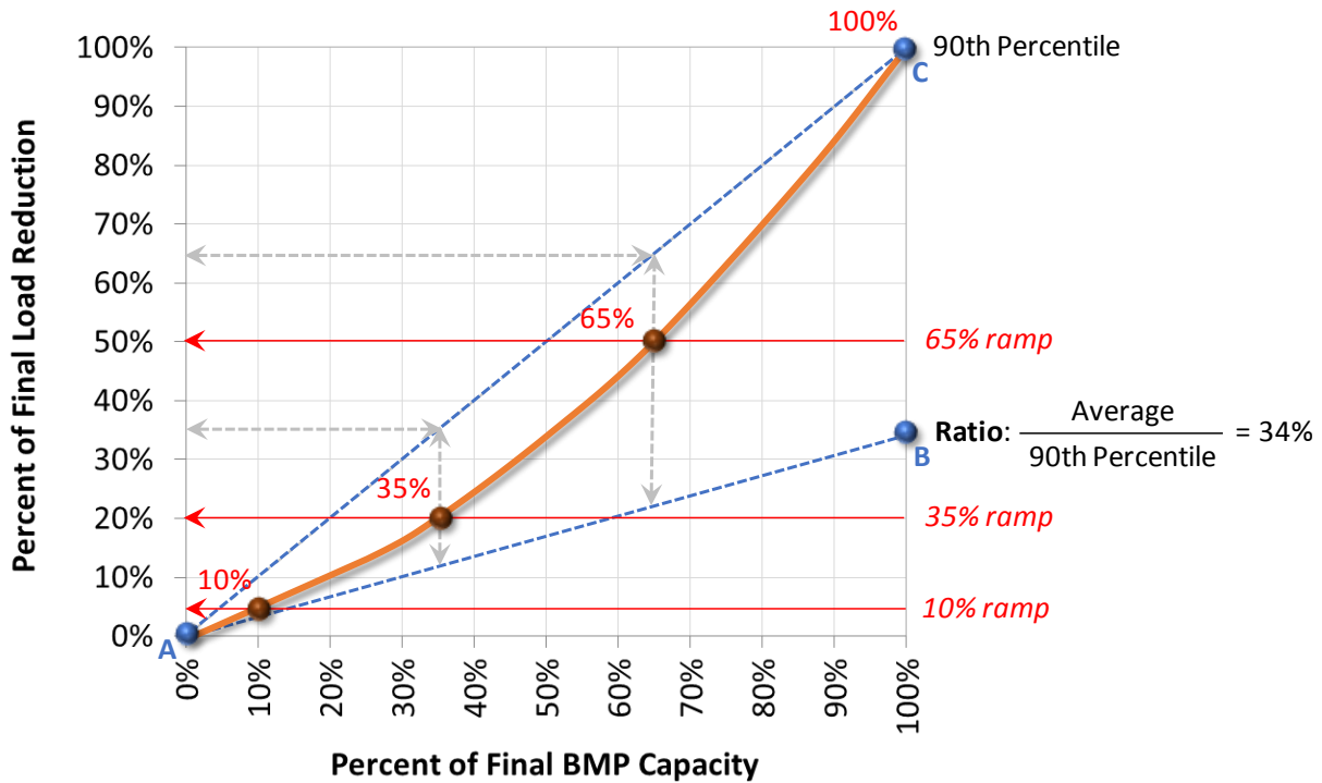
Figure 6-11 Illustration of Gradually Phasing from Average to Critical Conditions for Interim Milestones 1
