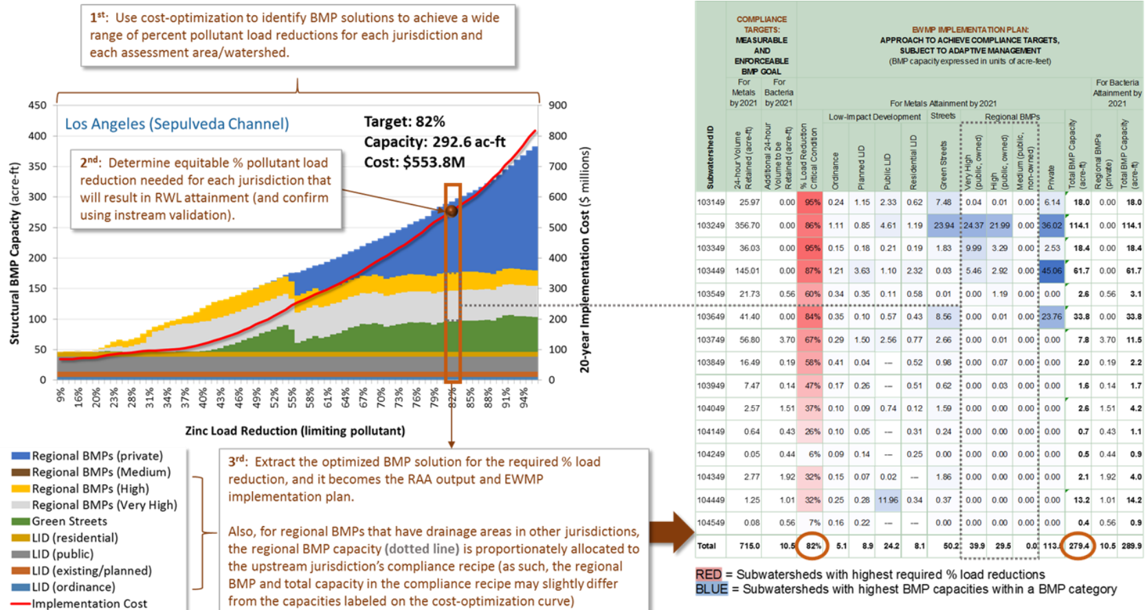
Figure 6-10 Illustration of How the EWMP Implementation Strategy is Extracted from a Cost Optimization Curve 1
