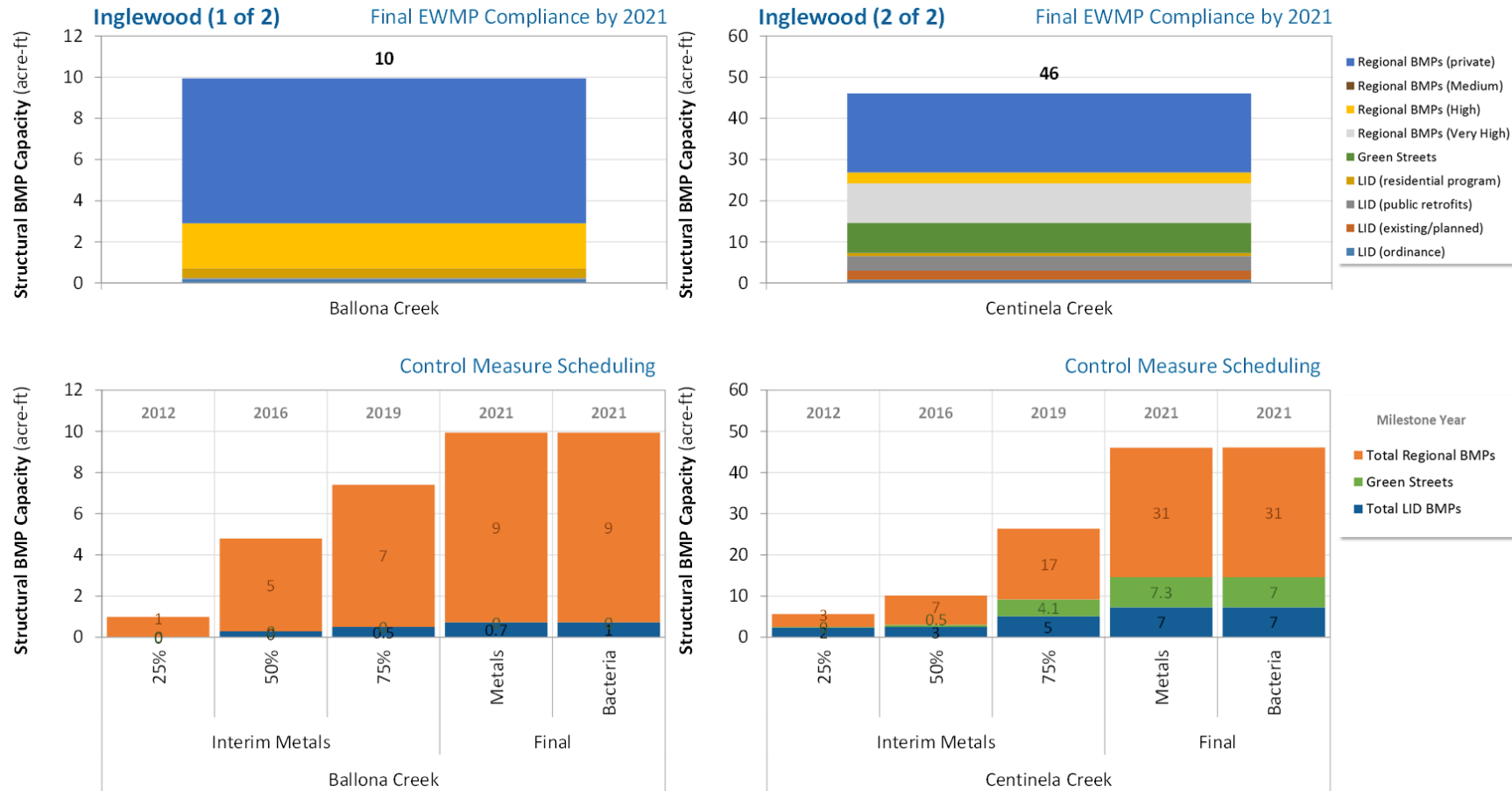
Figure 7-10 Inglewood: Scheduling of EWMP Implementation Strategy to Achieve EWMP/TMDL Milestones
