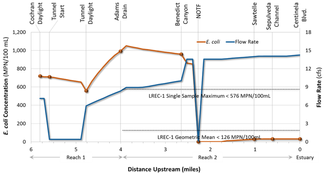
Figure 7-16 Concentration of E.coli in Ballona Creek with NOTF and Sepulveda Channel LFTF Operational
