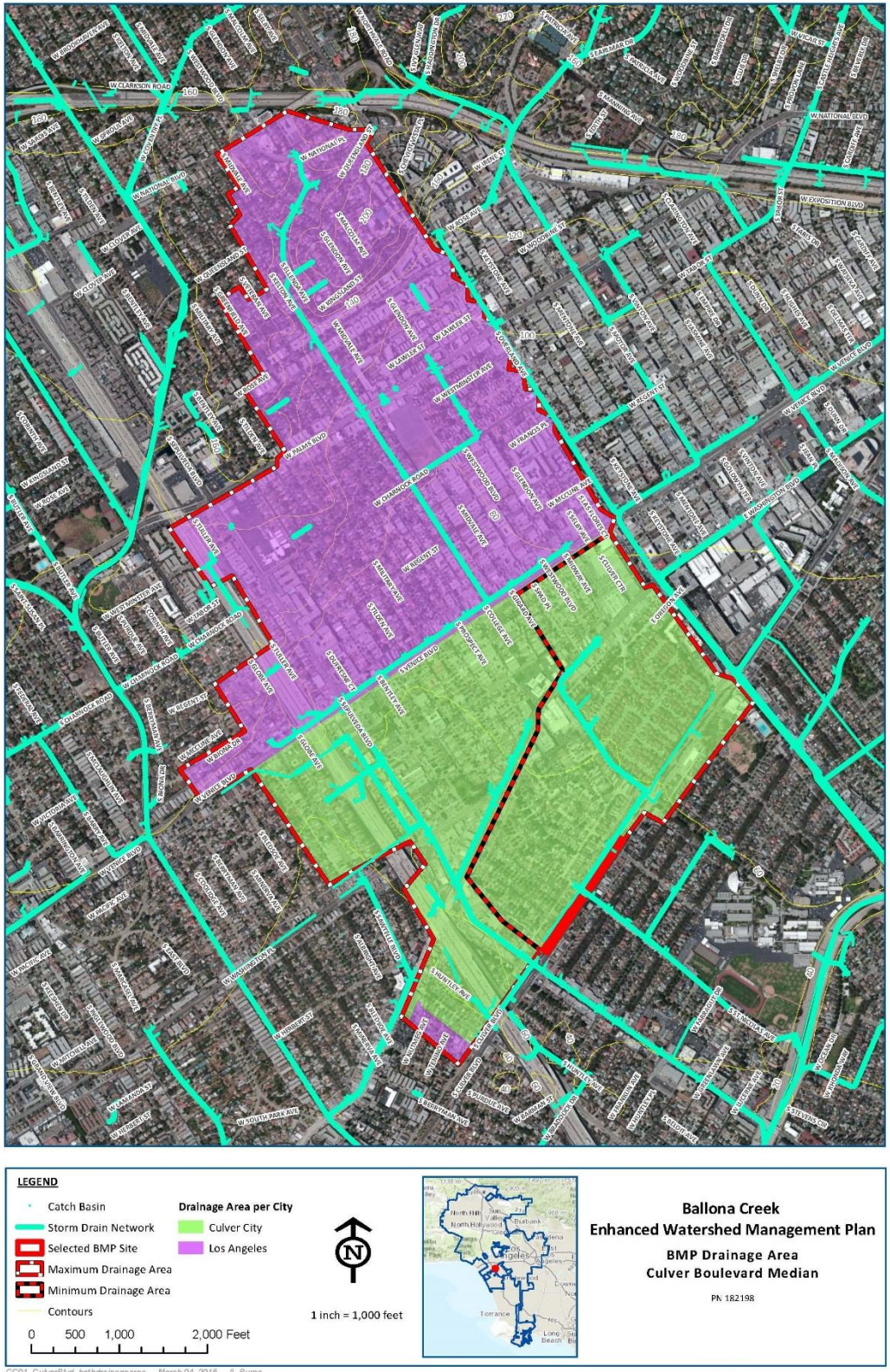
Figure 4-14 Culver Boulevard Median Subsurface Infiltration Drainage Area – Drainage Map
